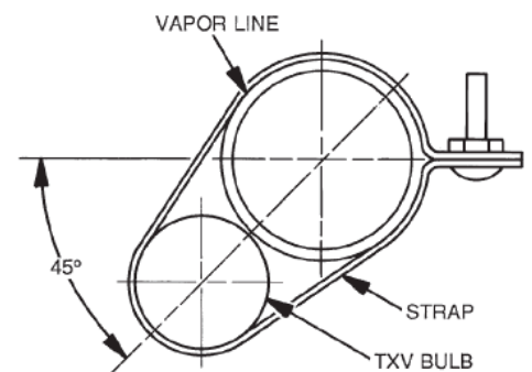
LEGEND TXV – Thermostatic Expansion Valve NOTE: The 8 o'clock position is shown above.
