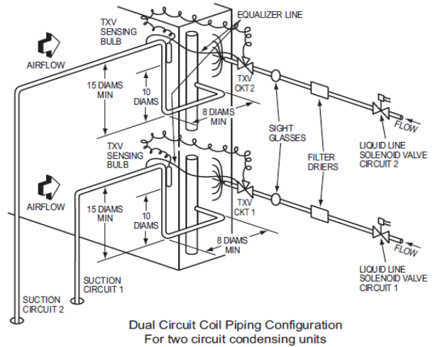
Dual Circuit Coil Piping Configuration RUM 10 - 16 For single compressor condensing units.
